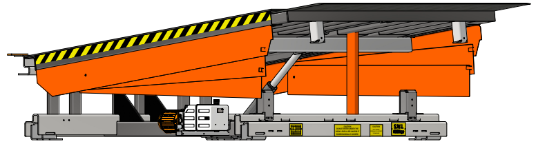
TELESCOPIC LIP
